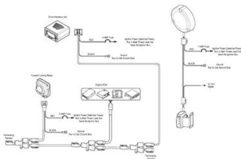
Collision Warning System with Side Object Detection
